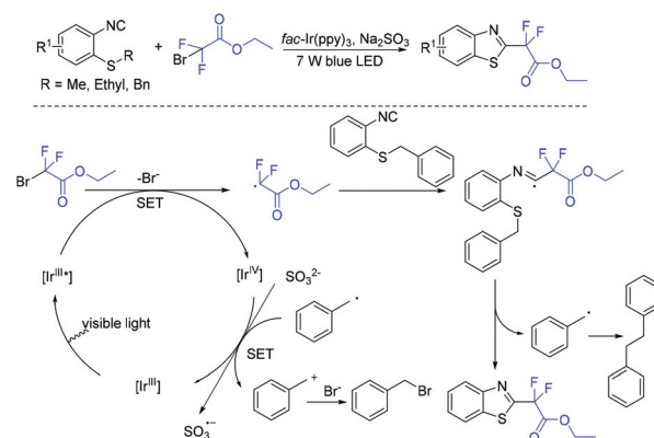
Scheme 108 The photocatalytic radical cascade cyclization of 2-isocyanarylthioethers.
