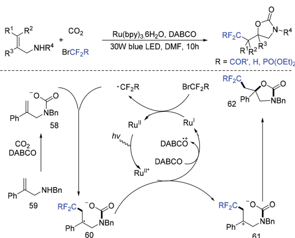
Scheme 34 The difluoroalkylation of allylamines with carbon dioxide.
