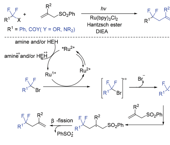
Scheme 57 The visible-light-induced coupling of difluoromethyl halides with allyl sulfones.
