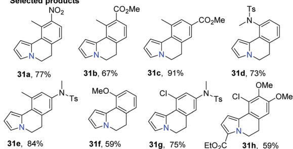
Scheme 4 Palladium-catalyzed alkylation/direct arylation sequence.
