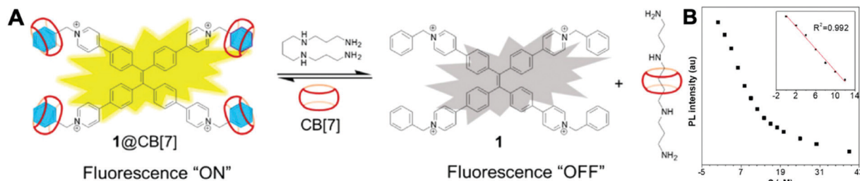
Fig. 13 (A) Proposed mechanism of fluorescent probes 1@CB[7] for spermine detection. (B) The fluorescence intensity of 1@CB[7] at 537 \text{ nm} as a function of the concentration of spermine ( 0-40 \mu M ). Inset shows the plot and linear fitting of fluorescence intensity at 537 \text{ nm} vs. the concentration of spermine ( 0-12 \mu M ). Adapted with permission from ref. 46. Copyright 2018 Elsevier B.V.
