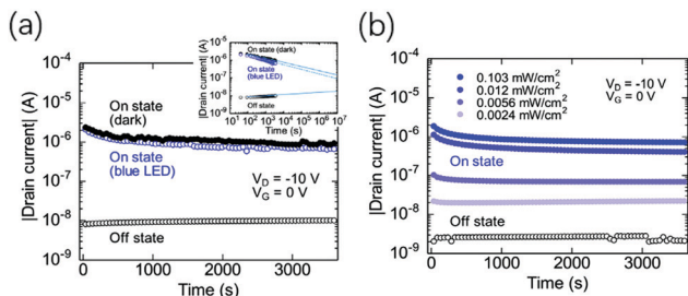
Fig. 15 (a) Retention curves of drain currents measured at V_G = 0 V and V_D = -10 V in the dark and under blue light illumination (469 nm, 1.06 mW cm -2 ) before and after programming with blue light. (b) Retention curves measured in the dark before and after programming ( V_G = +60 V, 3 s) with blue light at different intensities. Reproduced with permission. 90 Copyright 2019, Elsevier.
