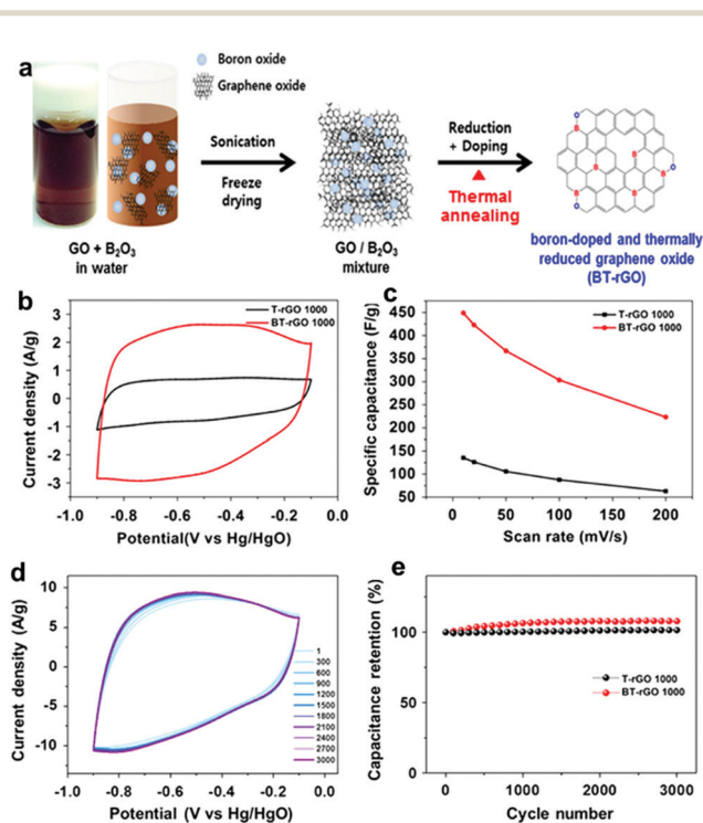
Fig. 20 (a) Schematic illustration of the preparation of BT-rGO. (b) CV curves at a scan rate of 10 mV s -1 . (c) Specific capacitances as a function of scan rate. (d) CV curves for 3000 cycles at a scan rate of 50 mV s -1 . (e) Capacitance retentions as a function of cycle number of T-rGO and BT-rGO electrodes. Reproduced with permission from ref. 138. Copyright 2015 Springer Nature.
