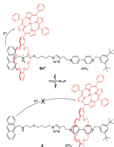
Fig. 6 [2]Rotaxane 6 with pH-switchable room temperature phosphorescence.
