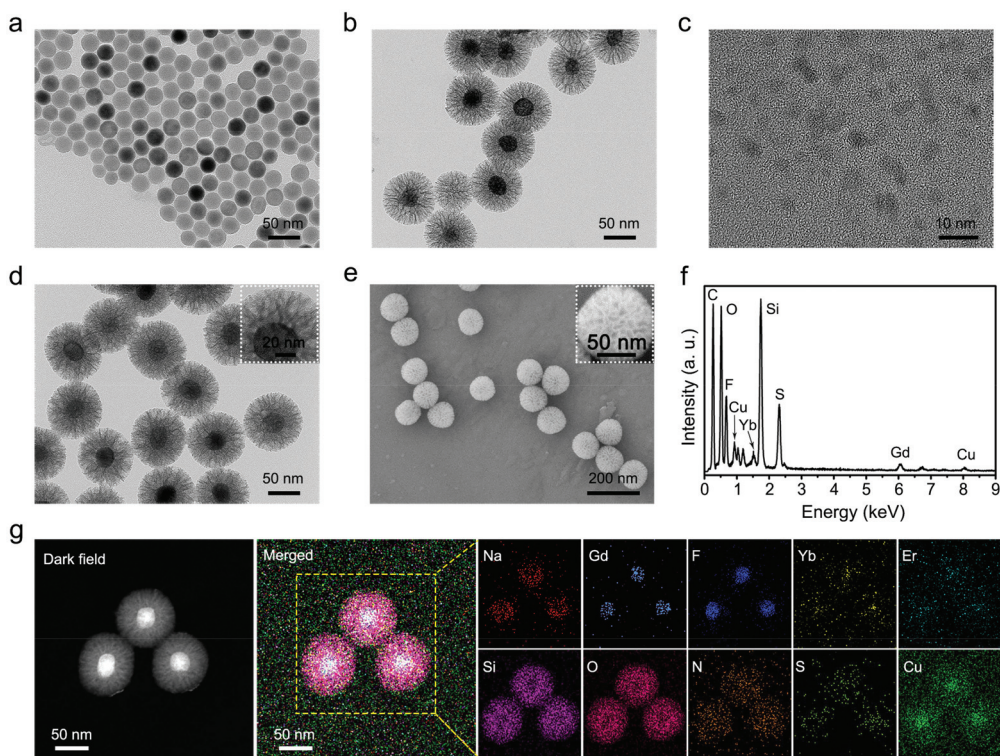
Fig. 1 Structural and compositional characterization of UMNOCC-PEG nanoparticles. TEM images of (a) the \text{NaGdF}_4:\text{Yb,Er} core nanoparticles, (b) UCNP@MSN-SNO, (c) \text{CuO}_2 nanodots, and (d) UMNOCC-PEG nanoparticles. (e) SEM image and (f) corresponding EDS spectrum of the UMNOCC-PEG nanoparticles. (g) Dark-field STEM image and the corresponding elemental mappings of UMNOCC-PEG nanoparticles.
