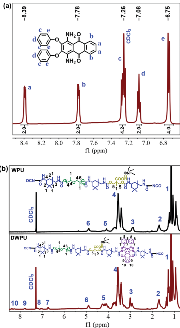
Fig. 7 ^1\text{H} NMR spectra of DV26 (a) and DWPU (b).
