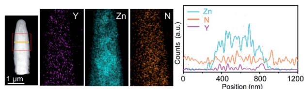
Fig. 7 TEM images of PCN coated Y:ZnO NRs and the corresponding distribution of the elements along the rods. Reproduced with permission from ref. 79 Copyright (2018) Wiley-VCH.
