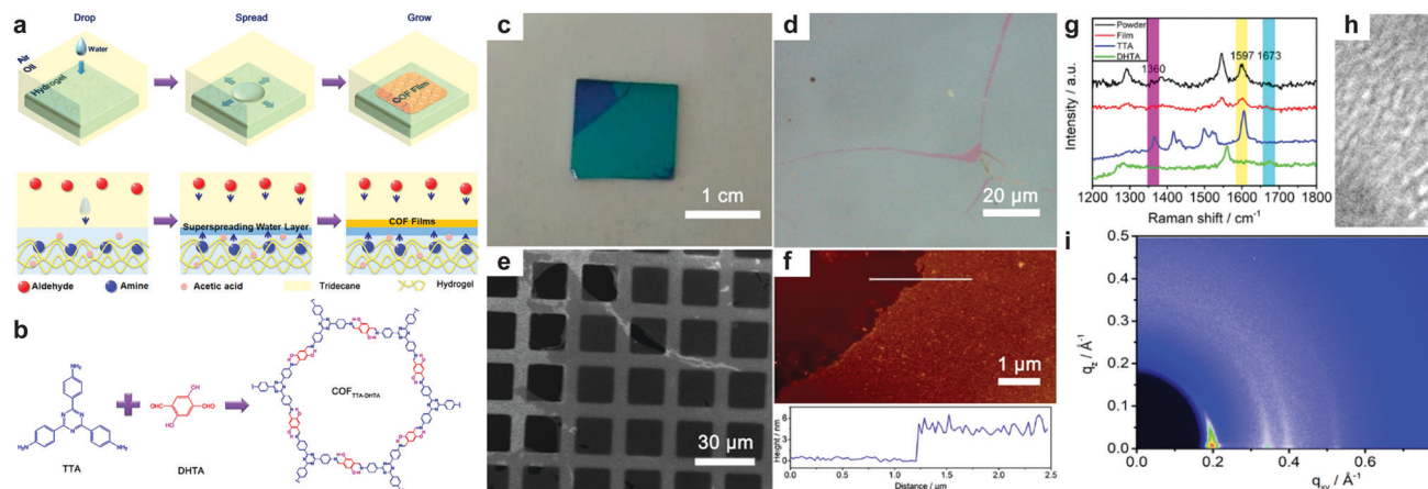
Fig. 35 (a) Scheme of triphase confined synthesis of COFenes. (b) Synthesis of COF TTA-DHTA . (c) Photo image of the COF TTA-DHTA film on a silica wafer. (d) Optical microscopic image of the COF TTA-DHTA film. (e) SEM image of the COF TTA-DHTA film on TEM grids. (f) AFM height image of the COF TTA-DHTA film on a silica wafer. (g) Raman spectra of the COF TTA-DHTA film and powder, and the monomers. (h) TEM images of the COF TTA-DHTA film. Inset: SAED pattern of the films. (i) GIWAXS of the COF TTA-DHTA thin film. Reproduced with permission from ref. 25. Copyright 2018. American Chemical Society.
