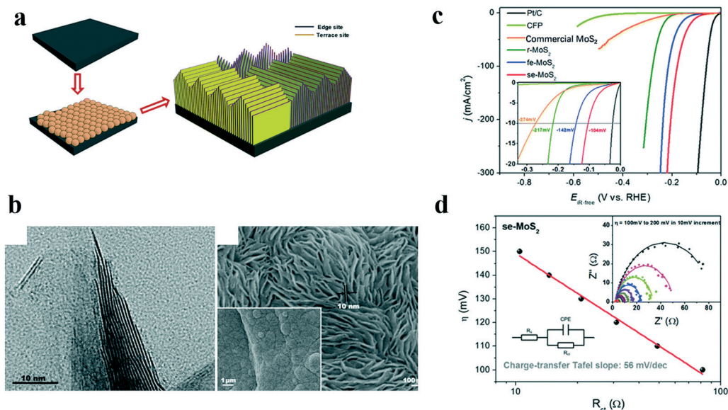
Fig. 6 Effects of high index faces on the catalytic performance of \text{MoS}_2 . 54 (a) Schematic illustration of stepped edge surface-terminated \text{MoS}_2 arrays (se- \text{MoS}_2 ). (b) HRTEM image of the se- \text{MoS}_2 layers showing that the crystal fringes of the S-Mo-S layers along the edge are stepped, (c) polarization curves and (d) charge-transfer Tafel plots of se- \text{MoS}_2 and control catalysts.
