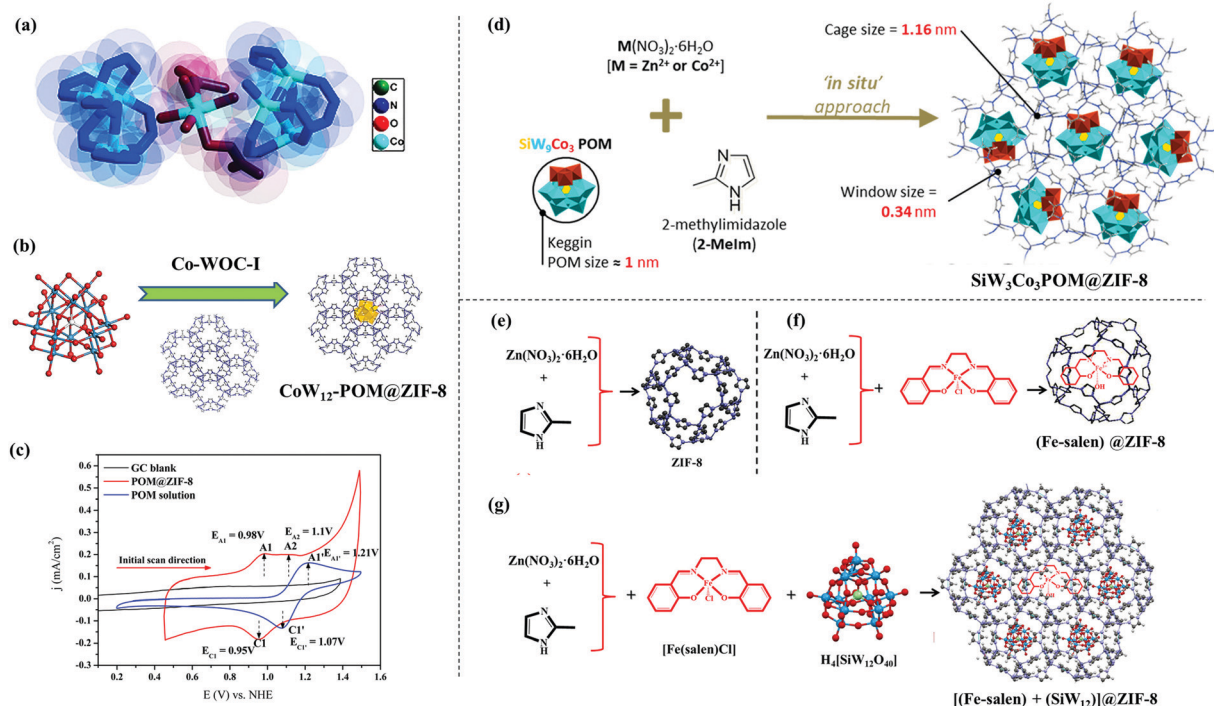
Fig. 3 (a) Active site structure of Co-WOC-1 . Adapted with permission from (ref. 108). Copyright (2016) John Wiley & Sons. (b) In situ encapsulation of [\text{CoW}_{12}\text{O}_{40}]^{5-} Keggin inside the ZIF-8 cavity; (c) cyclic voltammograms of POM@ZIF-8 and POM solution recorded in pH 2 0.1 M KCl; reprinted with permission from (ref. 109). Copyright (2018) John Wiley & Sons. (d) Synthetic protocol of SiW 3 Co 3 POM@ZIF-8 , reprinted with permission from (ref. 110). Copyright (2020) American Chemical Society. (e), (f), (g) Synthetic protocol of ZIF-8, Fe(salen)@ZIF-8 and [(Fe-salen) + (SiW 12 )]@ZIF-8 , respectively. Adapted with permission from (ref. 111). Copyright (2020) American Chemical Society.
