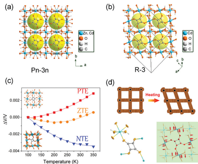
Fig. 11 Crystal structure of the cubic phase (a) and trigonal phase (b) of \text{MC}_4\text{O}_4 \cdot 2\text{H}_2\text{O} ( M = \text{Zn, Cd} ). (c) Temperature-dependent relative volume changes of the three compounds. (d) Scheme of the wine-rack distortion of the framework in the trigonal phase \text{Cd\_sq\_R} and illustration of the transverse vibration of the squarate ligand. Reprinted with permission from ref. 93.
