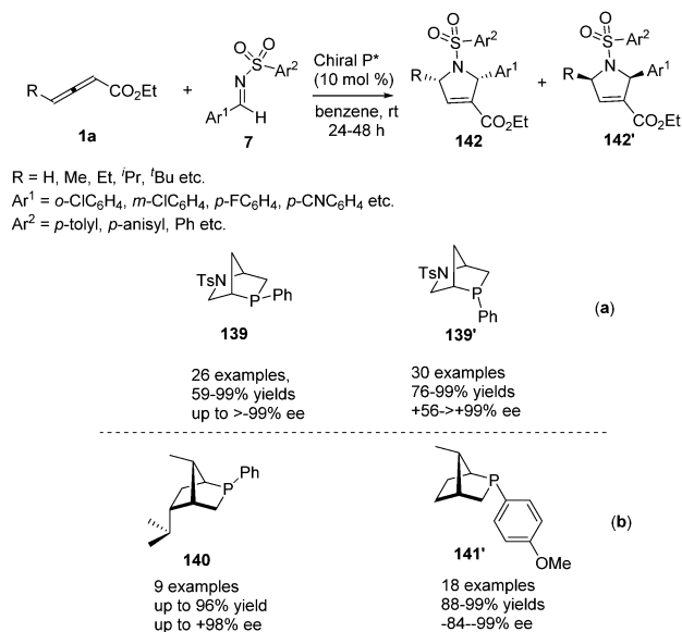
Scheme 45 Hydroxyproline-derived pseudoeantiomeric [2.2.1]bicyclic phosphines: asymmetric synthesis of (+)- and (-)-pyrrolines.
