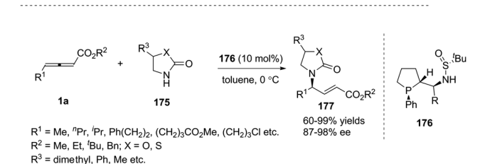
Scheme 54 Phosphine-catalysed \gamma -addition of substituted pyrazoles, imidazoles and oxazolidones.
