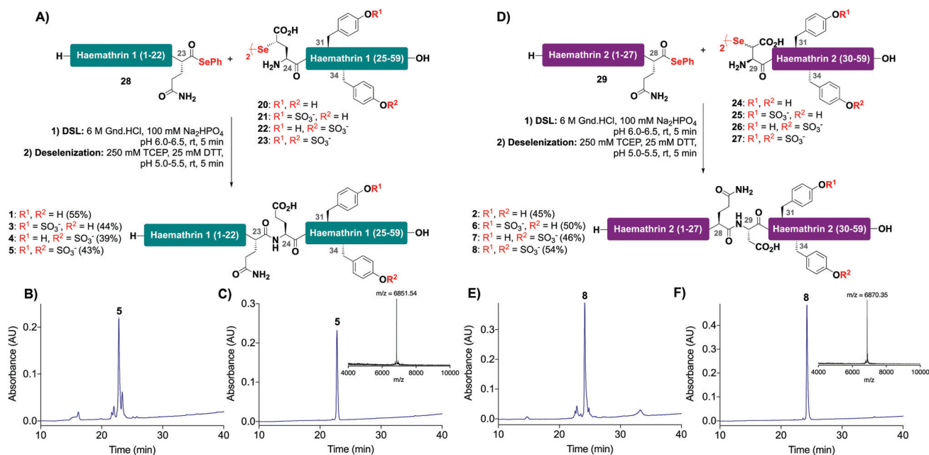
Scheme 2 Synthesis of haemathrin-1 and haemathrin-2 (sulfo)proteins 1 – 8 via a one-pot DSL-deselenization approach. (A) One-pot synthesis of haemathrin-1 variants 1 and 3 – 5 ; (B) HPLC chromatogram of crude DSL-deselenization reaction to afford doubly sulfated haemathrin-1 5 ; (C) HPLC chromatogram of purified doubly sulfated haemathrin-1 5 ( R_t = 22.8 min, gradient 0–50% B over 30 min, \lambda = 230 nm) with MALDI-TOF MS inset; (D) one-pot synthesis of haemathrin-2 variants 2 and 6 – 8 via DSL-deselenization; (E) HPLC chromatogram of crude DSL-deselenization reaction to afford doubly sulfated haemathrin-2 8 ; (F) HPLC chromatogram of purified doubly sulfated haemathrin-2 8 ( R_t = 24.2 min, gradient 0–50% B over 30 min, \lambda = 230 nm) with MALDI-TOF MS inset.
