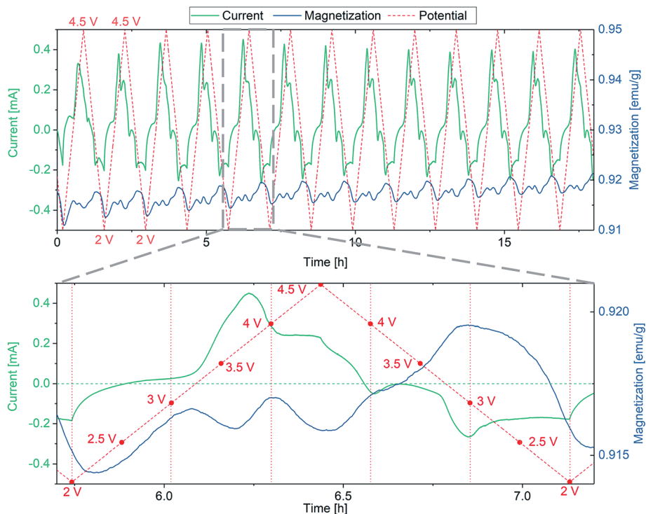
Fig. 1 First 13 cycles of the FeF 3 ·3H 2 O/Li insertion reaction (top) with a more detailed view of the 5 th cycle (bottom). CV/SQUID measurements showing the evolution of magnetization with current and potential. The sweep rate was 1 mV s -1 . The horizontal dashed green line in the bottom panel represents the zero line of current, while the vertical red dotted lines denote the potential at the respective time. Corresponding cyclic voltammograms can be found in the ESI (Fig. S2†).
