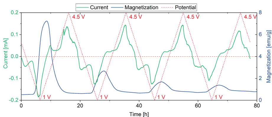
Fig. 2 Conversion reaction of FeF 3 ·3H 2 O. The sweep rate was set to 0.1 mV s -1 to account for the slow kinetics of conversion reactions in general. Magnetization degradation with cycling is observed, reflecting the decreasing appearance of Fe (0) .
