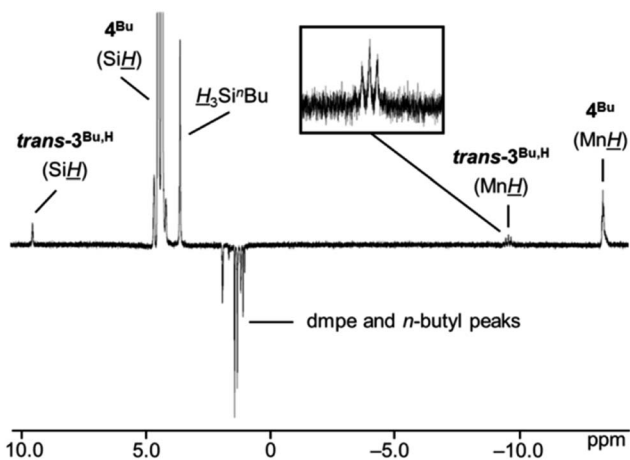
Fig. 6 1D NOESY/EXSY NMR spectrum of a solution of [(dmpe) 2 MnH(SiH 2 n Bu) 2 ] ( 4^{\text{Bu}} ) at 335 K with excitation at the SiH signal of 4^{\text{Bu}} , showing chemical exchange between the SiH and MnH environments of [(dmpe) 2 MnH(SiH 2 n Bu) 2 ] ( 4^{\text{Bu}} ) and trans -[(dmpe) 2 MnH(=SiH n Bu)] ( trans -3 Bu,H ), and the SiH environment of free \text{H}_3\text{Si}^n\text{Bu} . Positive (EXSY) peaks are indicative of chemical exchange and negative (NOESY) peaks are indicative of through-space coupling (500 MHz, \text{C}_6\text{D}_6 ).
