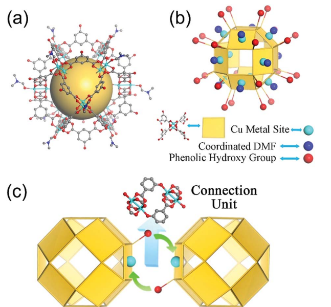
Fig. 1 The structure of discrete nanocage 1. (a) The ball-stick representation of nanocage 1; (b) the simplified structure of nanocage 1; (c) the orbicular connection unit between two neighboring nanocages.
