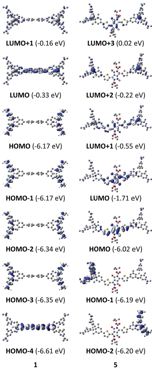
Fig. 2 DFT (CAM-B3LYP/6-31G(d))-calculated relevant orbitals for 1 and 5. Hydrogen atoms are omitted for clarity. Surface isovalue: \pm 0.03 [ e_0^{-3/2} ]. Orbital energy differences are not direct approximations of excitation energies. They are provided here for comparison between the compounds.
