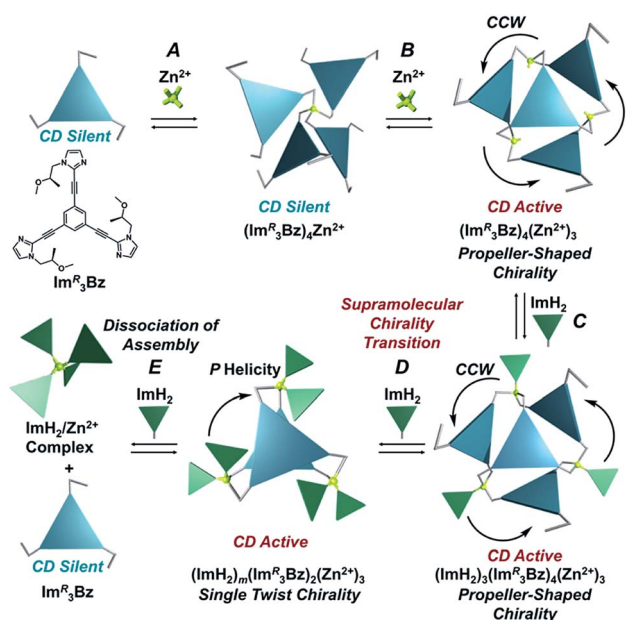
Scheme 3 Assembly formation of \text{Im}^{\text{R/S}}_3\text{Bz} with \text{Zn}^{2+} and \text{ImH}_2 .
