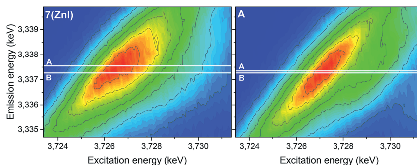
Fig. 11 U 3d4f RIXS spectra of complexes 7 (ZnI) and A. Lines A and B mark the energy positions of the maximum intensity of the resonant and normal emission, respectively.
