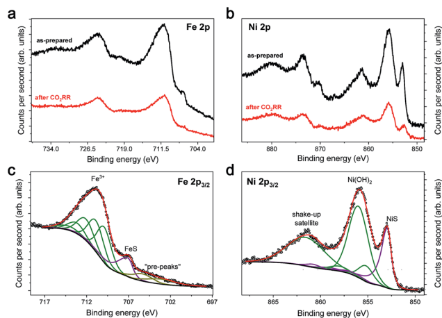
Fig. 4 (a) Fe 2p and (b) Ni 2p XPS spectra of pentlandite before and after CO 2 RR. Examples of the spectral deconvolution fit for the as-prepared sample are shown in (c) for the Fe 2p 3/2 core level and (d) for Ni 2p 3/2 .
