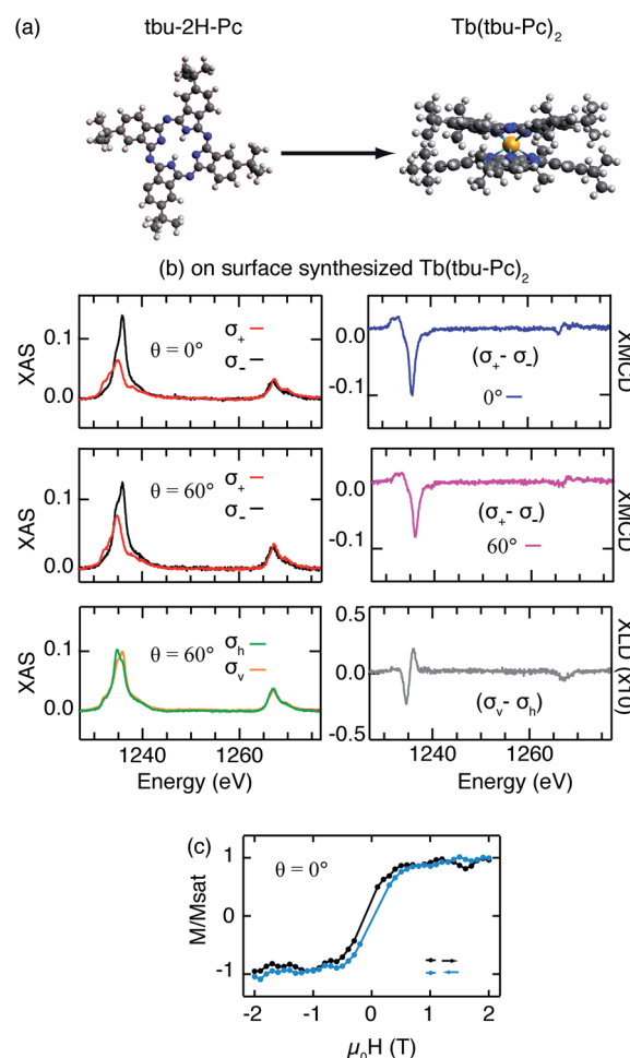
Fig. 5 (a) Schematic of tbu-2H-Pc and \text{Tb}(\text{tbu-Pc})_2 . (b) XAS, XMCD, and XLD probed at the Tb M_{4,5} edges and (c) magnetization curve probed at the Tb M_{4,5} edge (3.7 ML tbu-2H-Pc /Ag(111) + 0.8 ML Tb; \mu_0 H = 50 mT and 6.8 T for measurements with linear and circular polarizations, respectively, \mu_0 \dot{H} = 2 T \text{min}^{-1} for magnetization curves measurements, T = 3 K).
