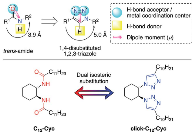
Fig. 1 Top: isosteric relationship between trans -amides and 1,4-disubstituted 1,2,3-triazoles. Bottom: double isosteric replacement of the LMW gelator C_{12} -Cyc investigated in this work.
