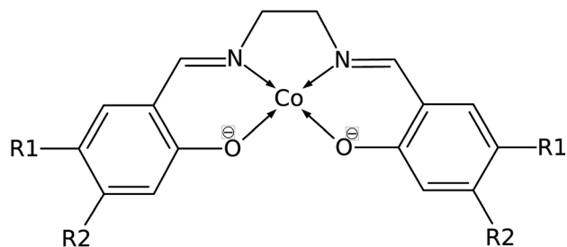
Fig. 2 Structure of Co(salen) ( R_1 = R_2 = \text{H} ), salen = N,N' -bis(salicylaldehyde)-ethylenediimino ligand. R_1 and R_2 are sites for substitution.
