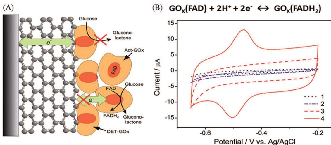
Fig. 4 (A) Schematic illustration of DET with GOx adsorption on the ERCGR/GOx/GCE. (B) CVs of the different modified GCEs; (1) bare GCE, (2) GOx/GCE, (3) ERGO/GCE, and (4) GOx/ERGO/GCE in \text{N}_2 -saturated phosphate buffer solution (PBS). [Reprinted with permission from ref. 190, B. Liang, X. Guo, L. Fang, Y. Hu, G. Yang, Q. Zhu, J. Wei and X. Ye, Study of Direct Electron Transfer and Enzyme Activity of Glucose Oxidase on Graphene Surface, Electrochem. Commun. , 2015, 50, 1–5. Copyright© Elsevier.]
