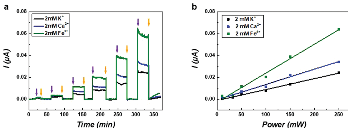
Fig. 4 (a) Real-time recordings of the ion current through the SLB on the integrated device by alternatingly switching on (purple arrows) and off (orange arrows) the hypersound (the input powers were successively 10, 32, 50, 100, 160, 250 mW). The electrolyte solutions were respectively KCl, \text{CaCl}_2 and \text{FeCl}_3 (2 mM in pure water). (b) Data points (markers) and linear fits (lines) of the ion current as a function of input power.
