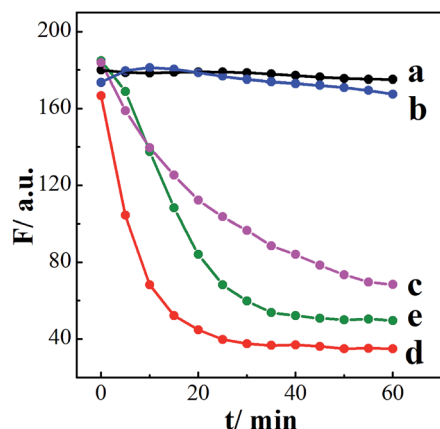
Fig. 4 Time-dependent fluorescence intensity changes of BDBA (a and d) and HBA (b and c) associated CDs in the absence (a and b) and presence (c and d) of \text{H}_2\text{O}_2 , and time-dependent fluorescence intensity changes of the CDs incubated with \text{H}_2\text{Q} (e).
