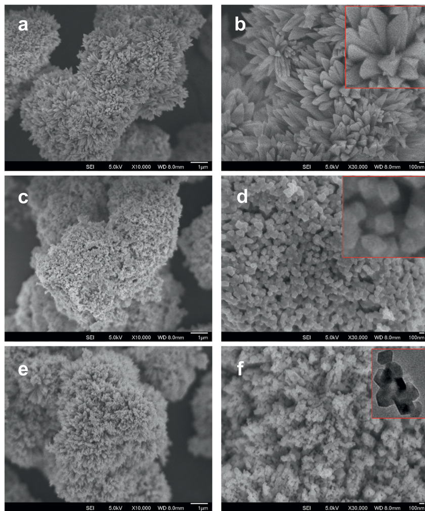
Fig. 2 SEM images: (a and b) [\text{Co/Ni}][\text{OH}]_2 , (c and d) \text{Co}_3\text{O}_4/\text{NiO} -400 °C, (e and f) \text{Co}_3\text{O}_4/\text{NiO} -600 °C microspheres at low and high magnifications. Scale bars: 1 \mu\text{m} in a, c, e; 100 nm in b, d, f.
