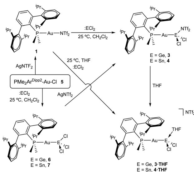
Scheme 1 Reactivity of tetrylene dihalides with gold compounds bearing a terphenyl phosphine.
