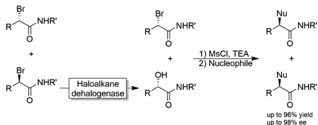
Scheme 30 Chemo-enzymatic enantioconvergent synthesis of optically active \alpha -substituted amides. Nucleophiles: Azide, benzylamine and phenol.
