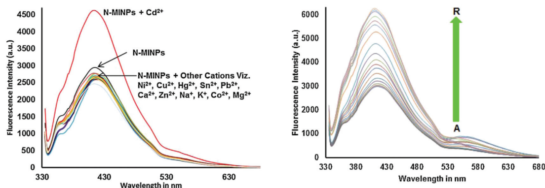
Fig. 11 Selectivity of 11 toward \text{Cd}^{2+} shows fluorescence enhancement as compared to other cations, and the fluorescence spectra of N -MNP suspension ( 1 \times 10^{-5} M) in the presence of different concentrations of \text{Cd}^{2+} ions. Adapted with permission from ref. 69. Copyright 2015 Elsevier Ltd.
