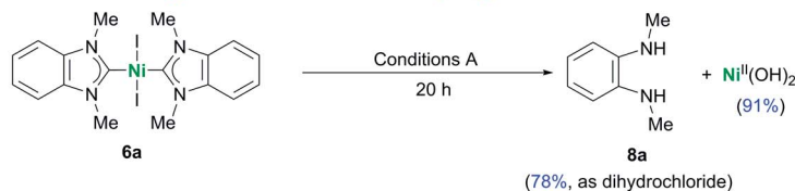
Scheme 3 Reactions of M/NHC complexes with KOH (Conditions A) and t-BuOK (Conditions B). HPLC and isolated (blue color) yields are shown for each case. HPLC/isolated yields are calculated assuming that, theoretically, 1 mole of azolone 7a , c , and f is formed from 1 mole of the complex 4a and b , and 6a and b . Conditions A: KOH , H_2O , pyridine, 100^\circ C ; Conditions B: t-BuOK , 1,4-dioxane, 100^\circ C . For additional details and other reaction conditions see the Experimental section, Table S1 and Fig. S1†
