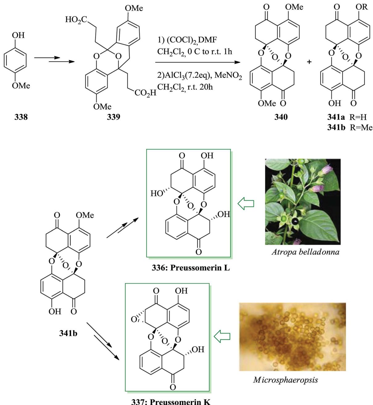
Scheme 69 Total synthesis of preussomerin L 336 and preussomerin K 337.
