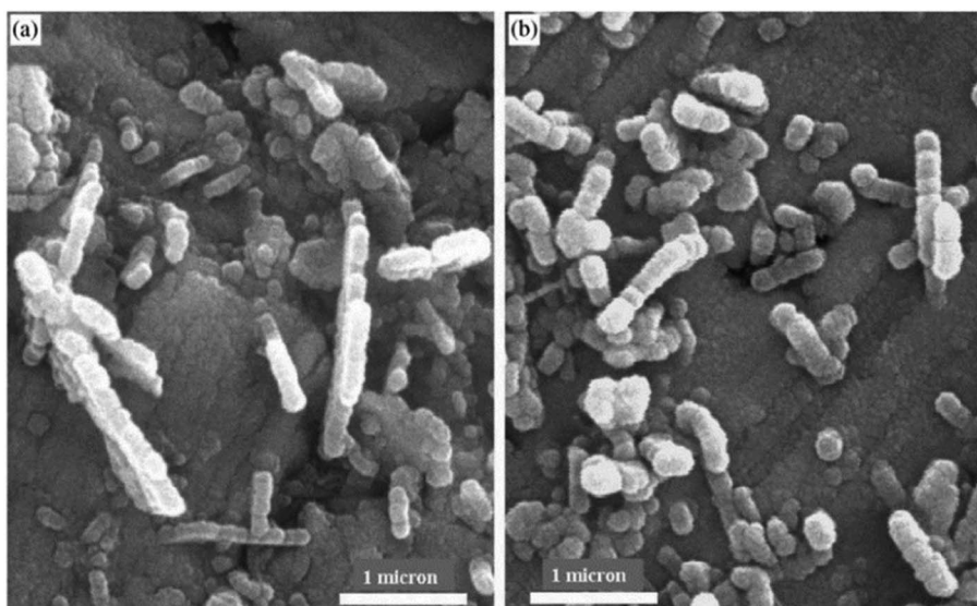
Fig. 14 SEM micrograph of \text{TiO}_2 nanowires deposited without \text{NH}_3 at 500\text{ }^\circ\text{C} ; (a) with 800 sccm argon flow, and (b) with 500 sccm argon flow. 163
