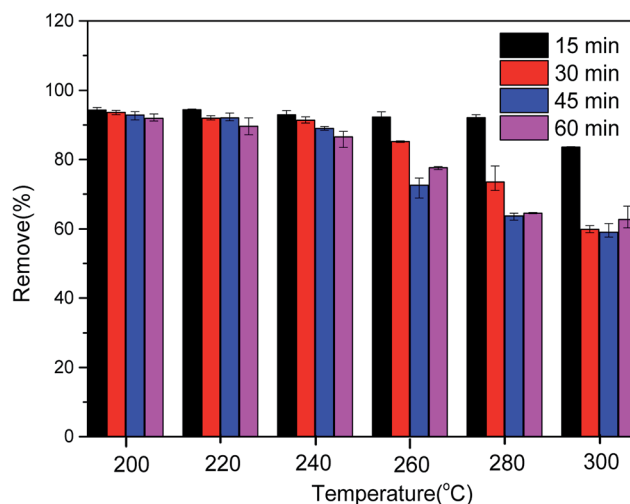
Fig. 3 Effect of torrefaction temperature and torrefaction time of CMB on removal rate. ( C_0 = 100 \text{ mg L}^{-1} , W = 0.01 \text{ g} , V = 20 \text{ mL} , t = 80 \text{ min} , T = 25^\circ\text{C} ).
