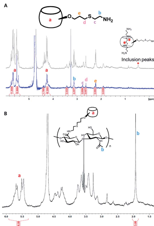
Fig. 2 ^1\text{H} NMR analysis for (A) mCB[6], the formation of its inclusion with spermine, and (B) mCB[6]-HA.
