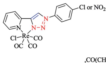
Scheme 27 Structure of the [(\text{C}_{13}\text{H}_9\text{N}_5\text{O}_2)\text{ReCO}_3\text{Cl (or NO}_2)] \cdot \text{CH}_3 \cdot \text{COCH}_3 complex.
