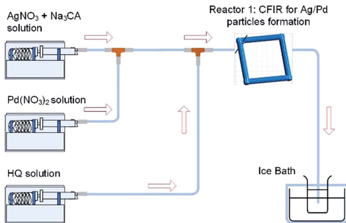
Fig. 11 Simultaneous reduction of Ag(NO 3 ) and Pd(NO 3 ) 2 with HQ in a CFI microreactor.
