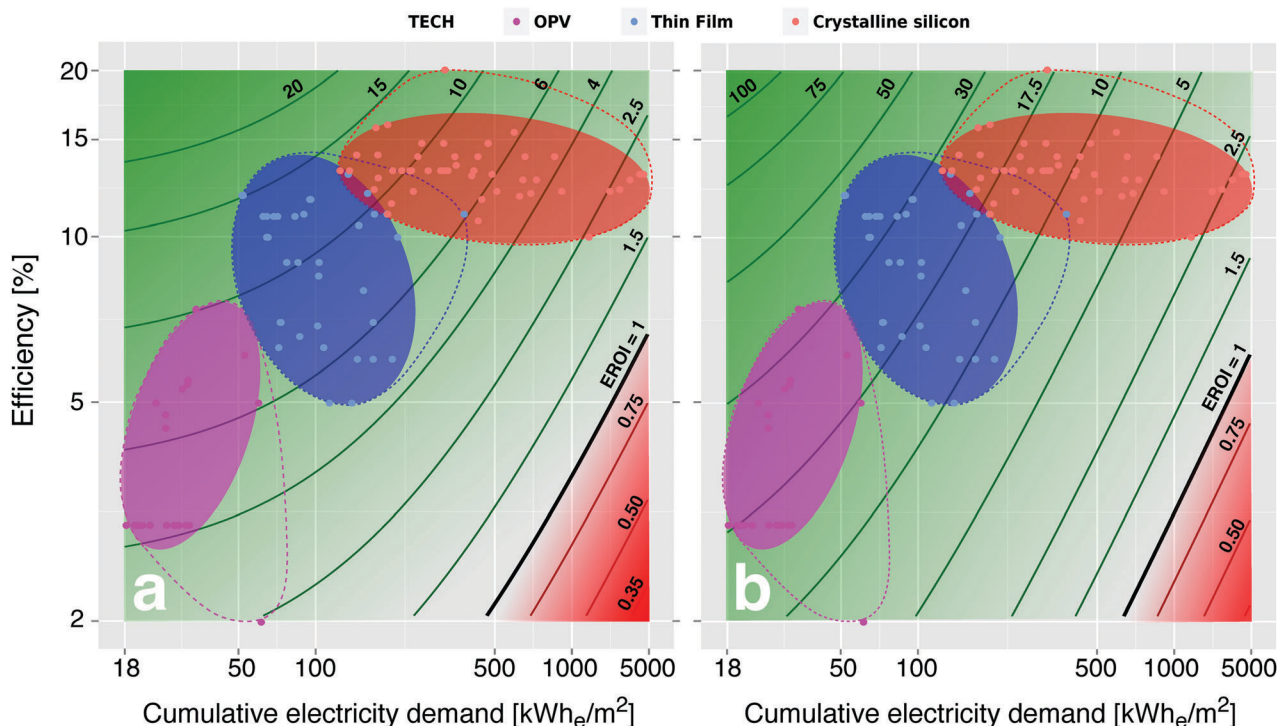
Fig. 3 PV system performance landscape (cumulative electricity demand, efficiency, and EROI) for different scenarios for the \text{CE}_e\text{D} of the balance of system (BOS). (a) A high BOS scenario, value 206 \text{kWh}_e/\text{m}^2 and (b) a low BOS scenario, value 37 \text{kWh}_e/\text{m}^2 . Outliers of each technology group are captured using a dashed line. As can be seen, the EROI is vastly different in the two scenarios; however, thin-film technologies (CdTe, CIGS, a-Si) perform best in both cases. The higher efficiency of the c-Si technologies (sc-Si, mc-Si) comes at the cost of a higher cumulative electricity demand for the total system.
