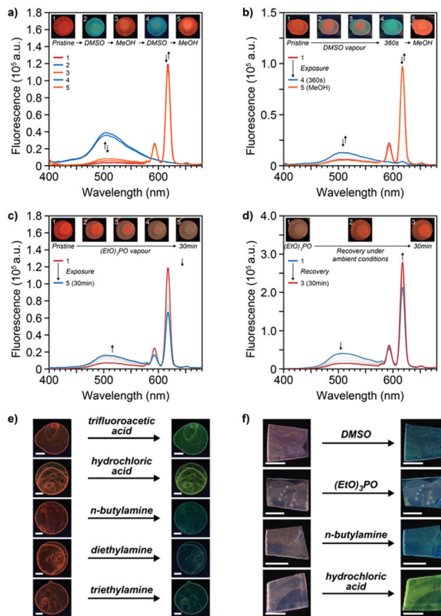
Fig. 4 Fluorescence spectra ( \lambda_{\text{ex}} = 370 \text{ nm} ) and pictures (all taken under illumination with 365 nm UV light) of drop-cast films of the MSP 2:Eu upon exposure to different analytes. (a) 2:Eu in its pristine state (1) and upon consecutive exposure to a drop of DMSO (2,4) and washing with MeOH (3,5). (b) 2:Eu in its pristine state (1) and upon exposure to DMSO vapours (2–4) for up to 360 s, followed by washing with MeOH (5) (spectra normalized at 617 nm). (c) 2:Eu in its pristine state (1) and upon exposure to (\text{EtO})_3\text{PO} vapour for up to 30 min (5). (d) Recovery of the sample shown in (c) under ambient conditions. (e) 2:Eu in its pristine state (left) and upon exposure to trifluoroacetic acid, hydrochloric acid, n -butylamine, diethylamine, as well as triethylamine (right). (f) 2:Eu on an ethylene vinyl alcohol copolymer support in its pristine state (left) and upon exposure to DMSO, (\text{EtO})_3\text{PO} , n -butylamine, and hydrochloric acid (right) (scale bar = 2 mm).
