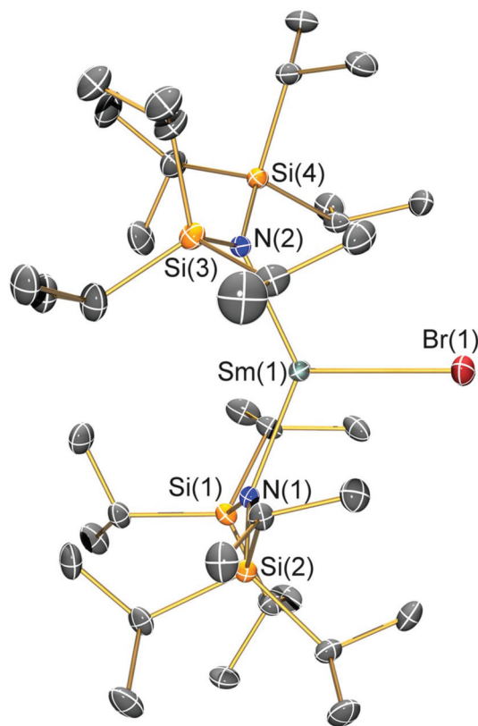
Fig. 3 Molecular structure of [\text{Sm}(\text{N}^{\dagger})_2]\text{Br} ( 2-Br ) with selective atom labelling. Displacement ellipsoids set at a 30% probability level and hydrogen atoms are omitted for clarity. Selected bond lengths [Å]: Sm(1)–Br(1) 2.7429(7), Sm(1)–N(1) 2.308(4), and Sm(1)–N(2) 2.324(4). Selected bond angles [°]: N(1)–Sm(1)–N(2) 133.52(14), N(1)–Sm(1)–Br(1) 112.19(10), and N(2)–Sm(1)–Br(1) 113.19(10).
