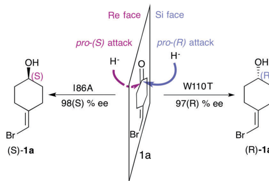
Scheme 1 Representation of the pro-( R ) and pro-( S ) hydride attack for substrate 1a , together with the experimentally reported enantioselectivity of the engineered variants TbADH W110T and TbADH I86A by Reetz and coworkers. 93
