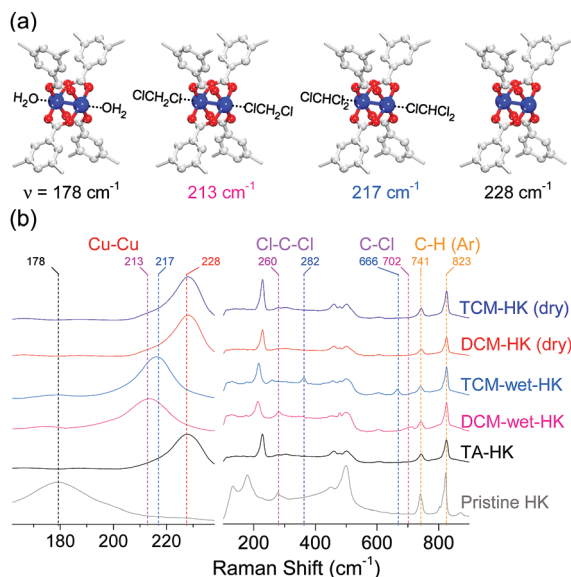
Fig. 2 (a) Schematics of H 2 O-coordinated, DCM-coordinated, TCM-coordinated, and open-state ( \text{Cu}^{\text{II}}_2 ) centers in HKUST-1 (from left to right). (b) Narrow (left) and wide (right) views of Raman spectra of pristine-HK (gray), TA-HK (black), DCM-wet-HK (pink), TCM-wet-HK (sky blue), dry DCM-HK (red), and dry TCM-HK (blue). Reprinted (adapted) with permission from ref. 70. Copyright (2018) American Chemical Society.
