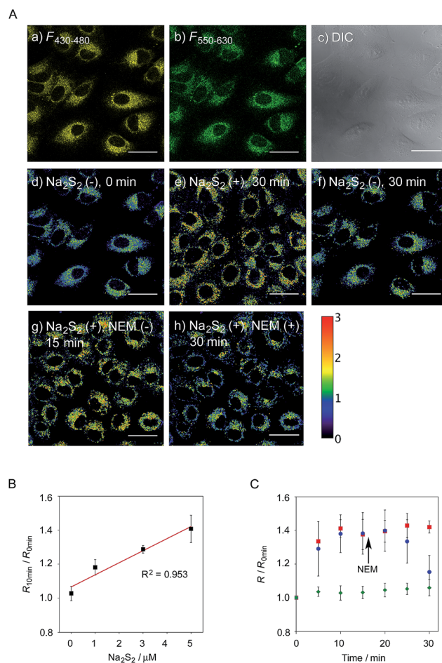
Fig. 4 (A) Fluorescence images of A549 cells treated with 6 -AM (5 \mu\text{M} ). (a) F_{430-480} , (b) F_{550-630} , (c) DIC, and (d) ratio image ( R = F_{430-480}/F_{550-630} ). (e and f) Ratio image after 30 min in the presence and absence of \text{Na}_2\text{S}_2 (5 \mu\text{M} ), (g and h) ratio image after 15 min in the presence \text{Na}_2\text{S}_2 (5 \mu\text{M} ) and subsequent treatment with NEM (100 \mu\text{M} ) for 15 min. Scale bar: 30 \mu\text{m} . (B) Ratio value change of A549 cells upon the addition of various concentrations of \text{Na}_2\text{S}_2 (0–5 \mu\text{M} ), n = 6 . (C) Time trace plot of the ratio value in A549 cells upon the treatment with \text{Na}_2\text{S}_2 (5 \mu\text{M} ) (red square, n = 6 ), \text{Na}_2\text{S}_2 (5 \mu\text{M} ) and the subsequent addition of NEM (100 \mu\text{M} ) at 15 min (blue circle, n = 4 ), without \text{Na}_2\text{S}_2 and NEM (green diamond, n = 6 ).
