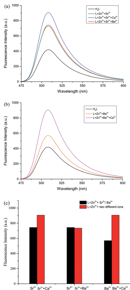
Fig. 6 (a) Fluorescence spectra of complex 2 solution ( 1.0 \times 10^{-5} \text{ mol L}^{-1} ) in the absence and presence of various metal ions (1.0 equiv. of Ca(II) and Ba(II)). (b) Fluorescence spectra of complex 3 solution ( 1.0 \times 10^{-5} \text{ mol L}^{-1} ) in the absence and presence of various metal ions (1.0 equiv. of Ca(II)). (c) Fluorescence response of L–Zn(II) solution ( 1.0 \times 10^{-5} \text{ mol L}^{-1} ) to various metal ions. ex = 367 nm, em = 508 nm.
