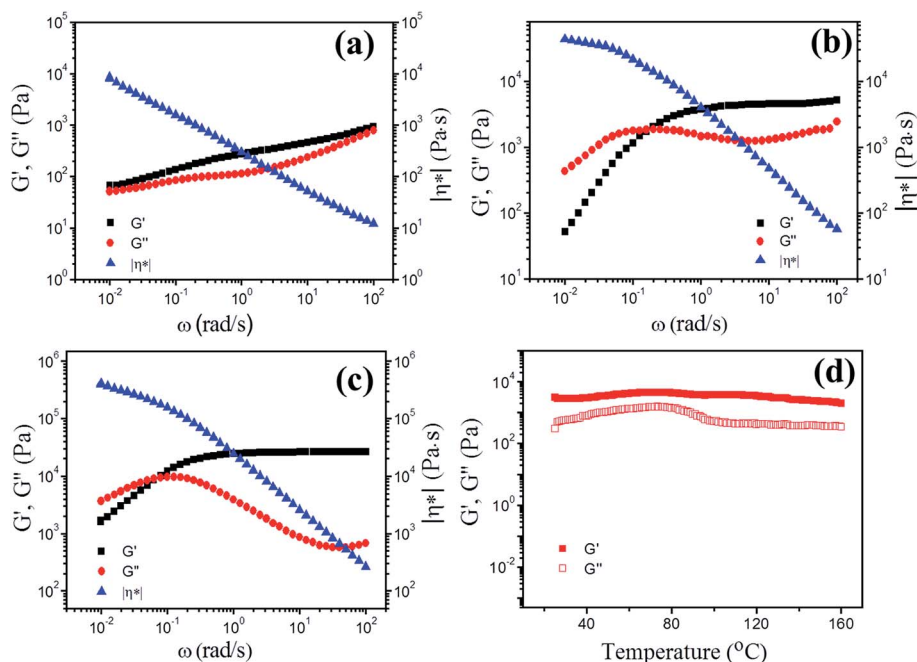
Fig. 4 G' , G'' , and |\eta^*| as functions of \omega at 25 °C for ionogels with different contents of PAMAM G1: (a) 10%, (b) 20%, and (c) 30%. (d) G' and G'' as functions of temperature at an angular frequency of 6.28 \text{ rad s}^{-1} for ionogel with 20% PAMAM G1.
