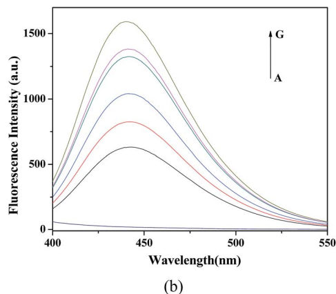
Fig. 8 (a) The reaction of TA with •OH. (b) Fluorescent spectra of acetate buffer solution (pH = 4) containing only TA and PDI-CuO (A) or with H 2 O 2 (0.25 M), TA (0.5 mM) and the PDI-CuO nanocomposites with different concentration ((B) 0, (C) 20, (D) 80, (E) 200, (F) 250, (G) 300 μg mL -1 ) were incubated at 55 °C for 30 min. The FL excitation wavelength was fixed at 315 nm.
