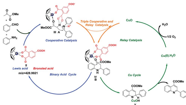
Scheme 4 Proposed mechanism of zirconocene dichloride/trimellitic acid/CuO cooperative and relay catalysis for synthesis of substituted quinolones.
