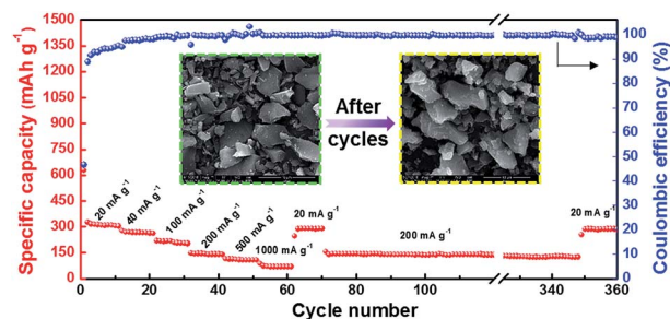
Fig. 8 Discharge capacities of HC-1000 at different current densities of 20, 40, 100, 200, 500 and 1000 \text{mA g}^{-1} , respectively. A long-term cycling performance is recorded from the 70 th to the 350 th cycles at 200 \text{mA g}^{-1} and SEM images of the HC-1000 electrodes before and after 360 cycles.
